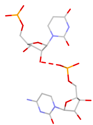
U:C S(sp:O2*-O2P)
