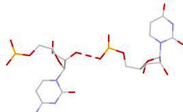
U:C rpS(ps:O1P-O2*)_2
