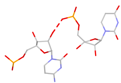
U:C rpS(ps:O1P-O2*)_1
