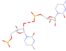
C:C rpS(ps:O1P-O2*)_2
