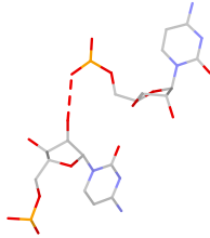
C:C rpS(ps:O1P-O2*)_1
