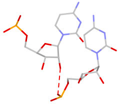
C:C pS(sp:O2*-O2P)
