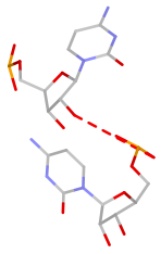
C:C S(sp:O2*-O1P)
