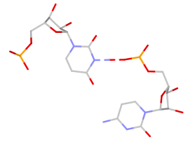
U:C rS*(bp:N3-O2P)
