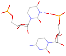
U:C S(bp:N3-O2P)
